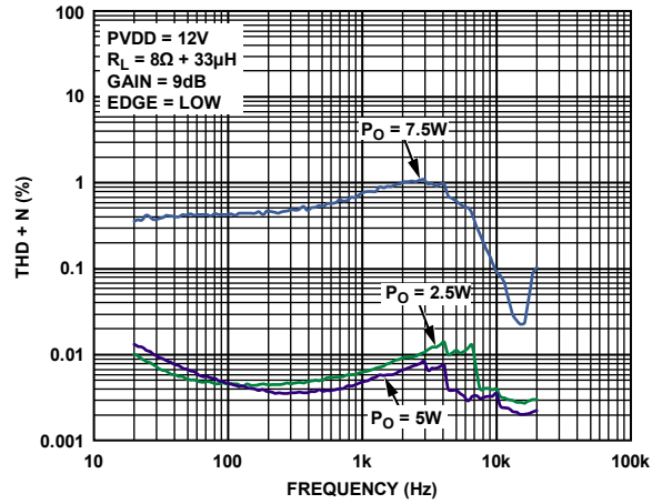
Figure 12. THD + N vs. Frequency; R_L = 8\Omega ; PVDD = 12V; P_O = 2.5W , P_O = 5W , P_O = 7.5W
